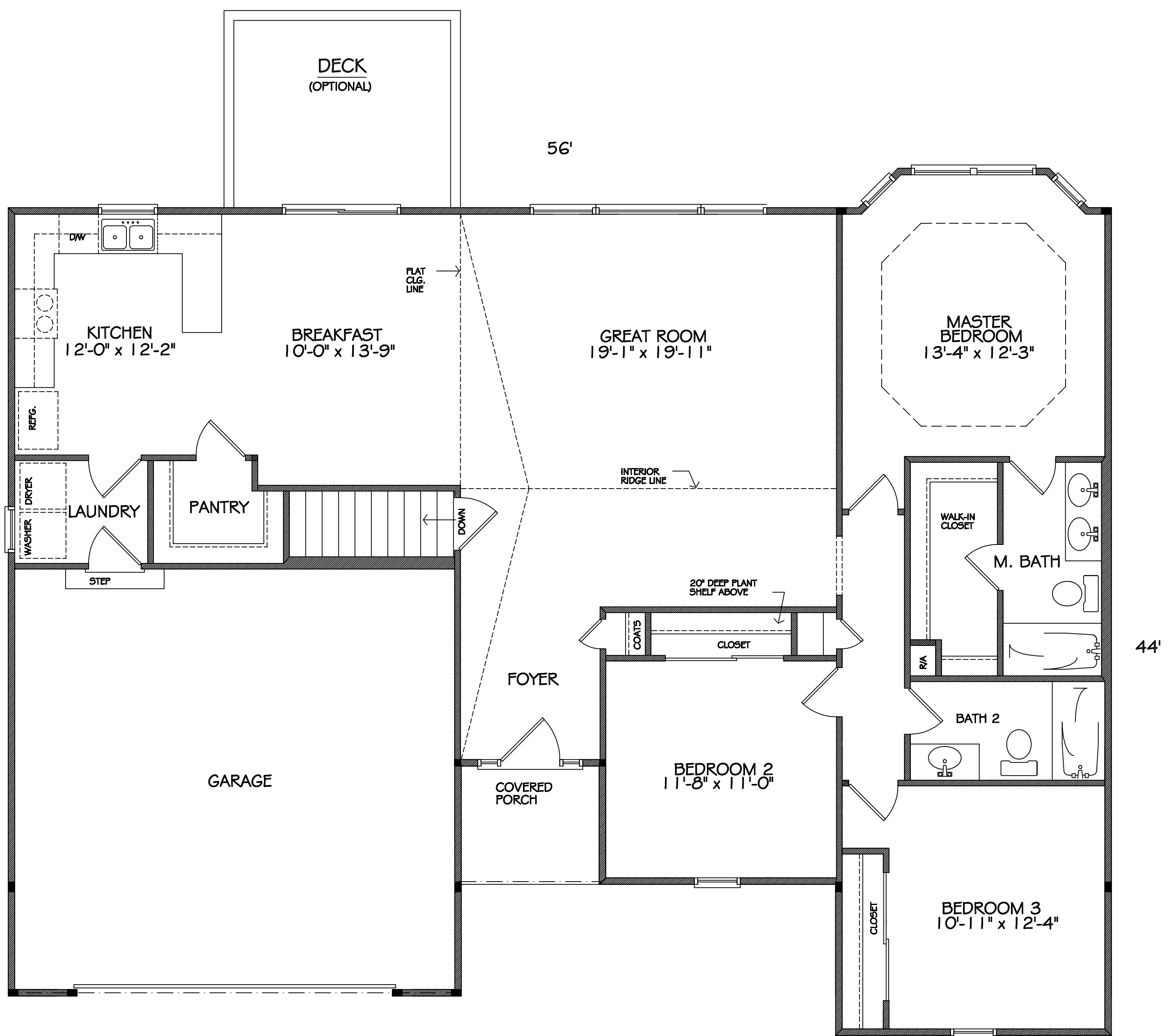
"HICKORY 2 BASEMENT" FLOOR PLAN 1650 SQ. FT.
