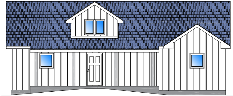
FRONT ELEVATION
