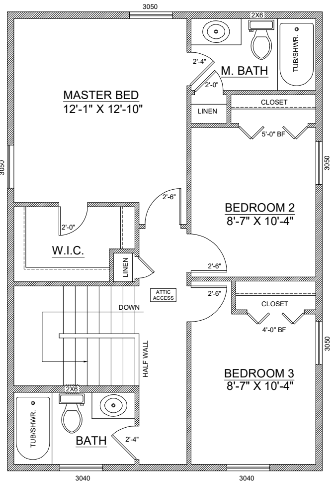
SECOND FLOOR
